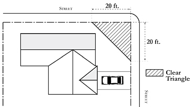
Fig. 18.08-1, Clear Vision Triangle
